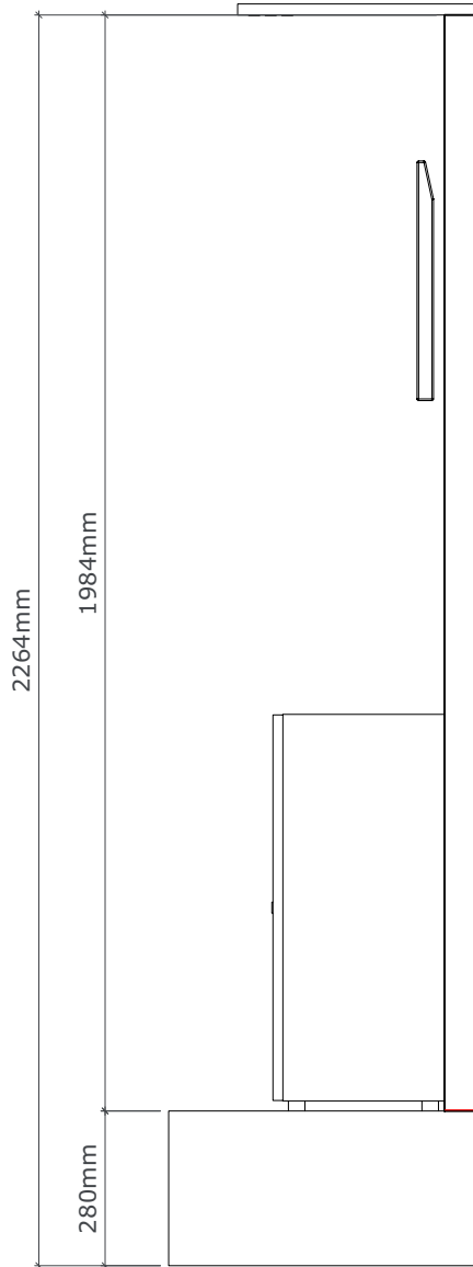
SIDEVIEW plinth max. weight 100kg
