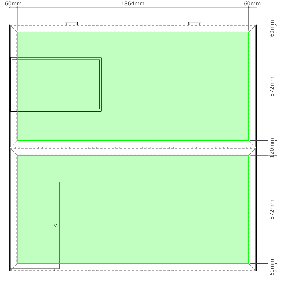
FRONTVIEW possible zones for fixating products only on request (max. weight 10kg)
